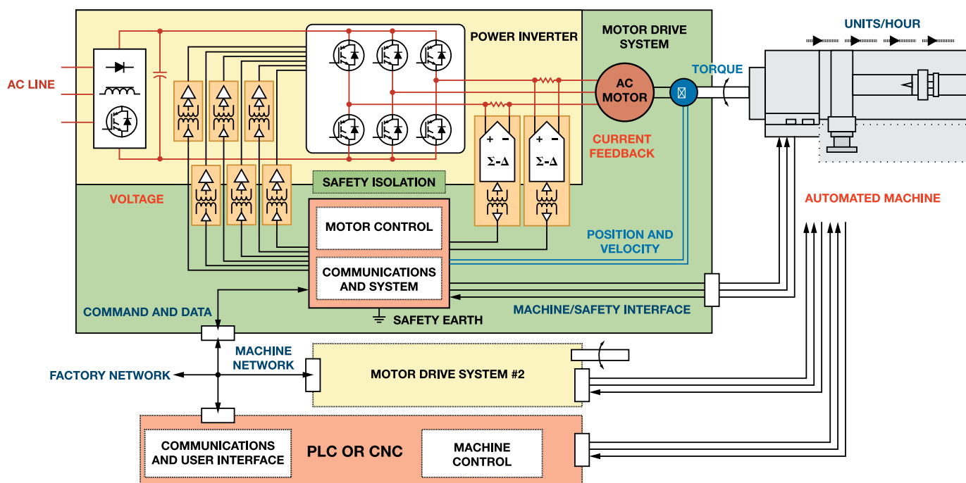
Figure 1: Block diagram of automated machine control system
